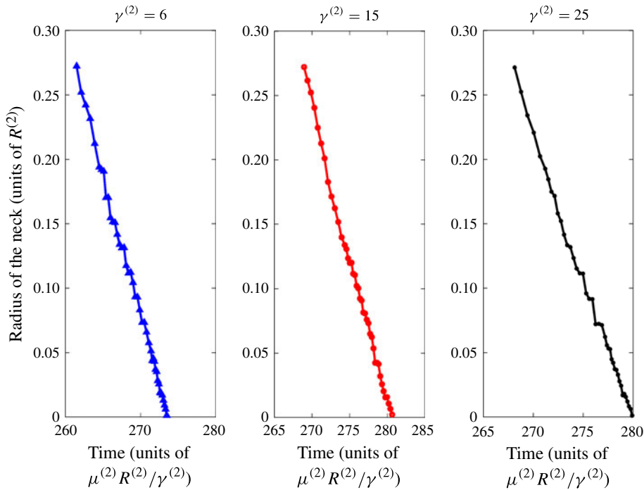
FIGURE 7. (Colour online) Radius of the fluid neck versus time during the final phase of the breakup of the outermost interface, from the three-dimensional Stokes simulations of figure 6. This breakup is asymptotically linear with time, similar to the predictions of the scaling theory for N = 2 systems (Lister & Stone 1998; Cohen et al. 1999).
